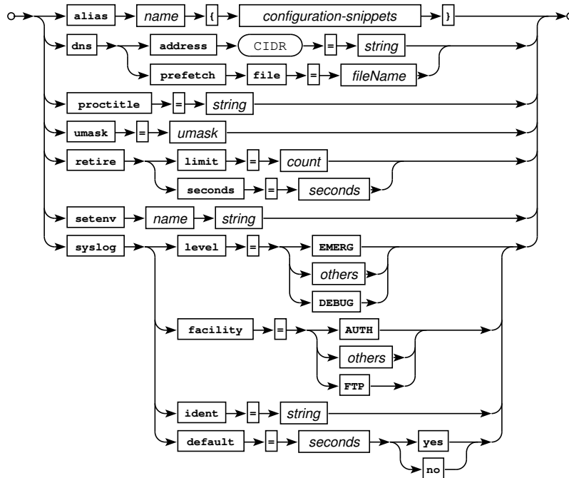
Railroad diagram: TopLevelAttr
