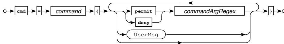
Railroad diagram: ShellCommandDecl
