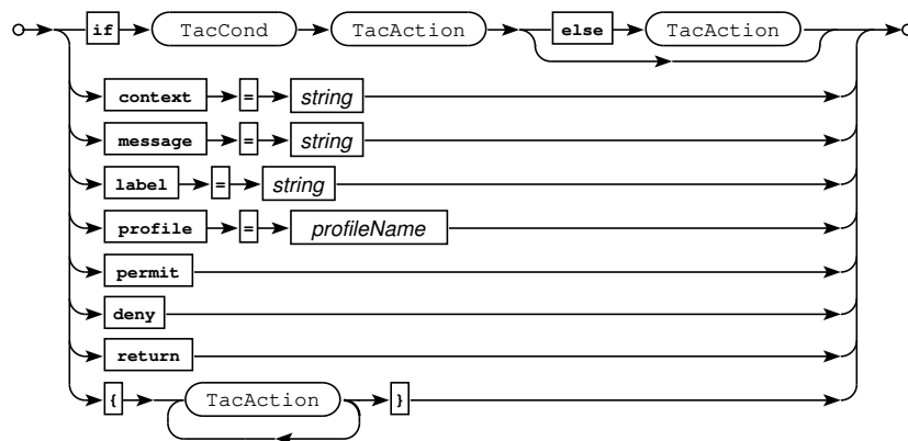
Railroad diagram: TacAction
