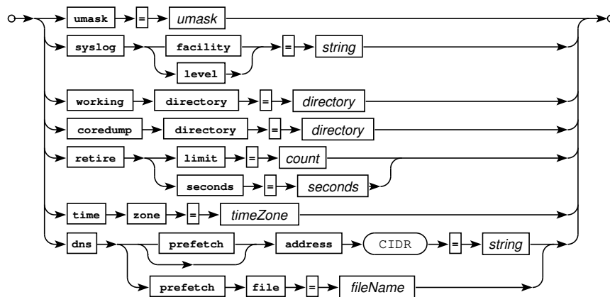
Railroad diagram: GlobalDecl
