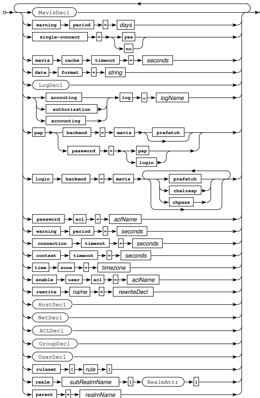
Railroad diagram: RealmAttr
