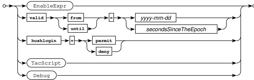
Railroad diagram: ProfileAttr
