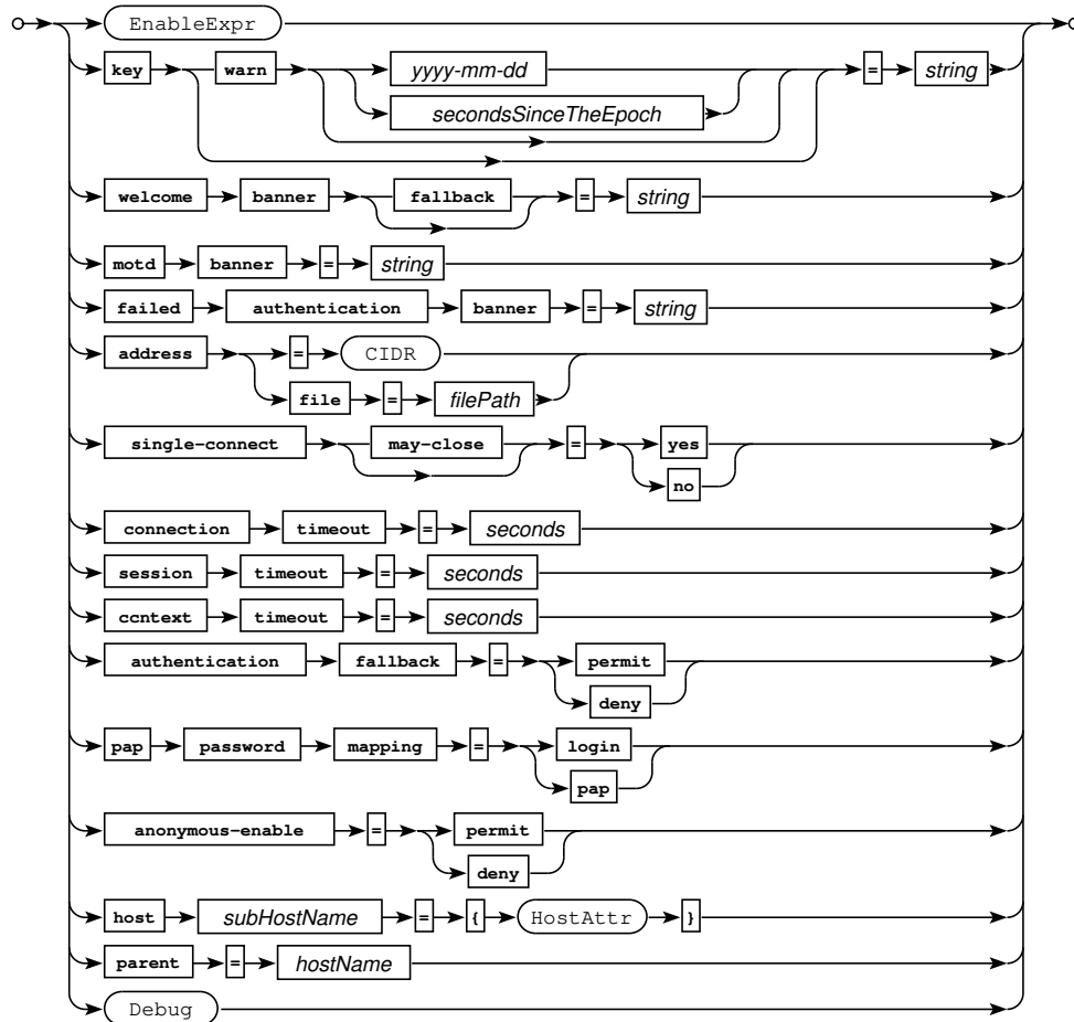
Railroad diagram: HostAttr
