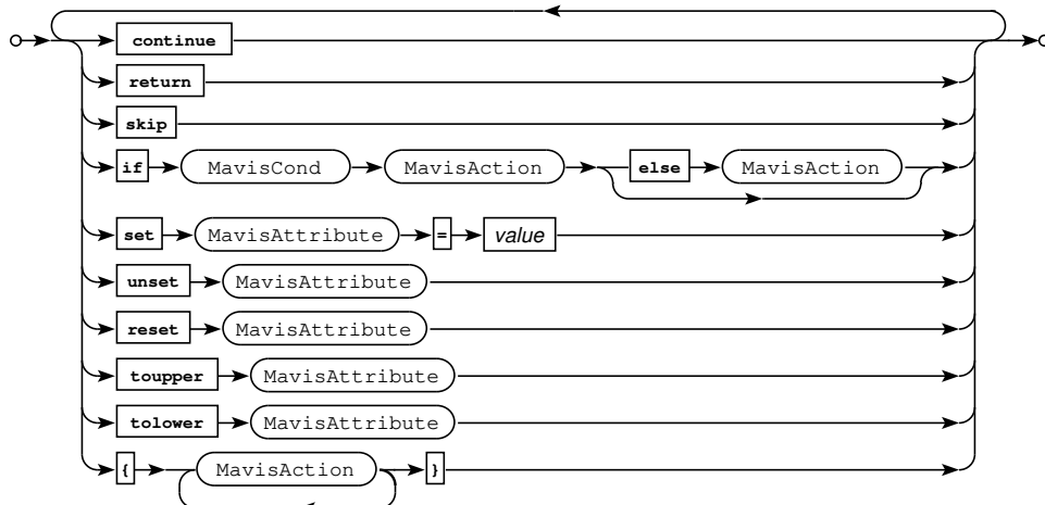
Railroad diagram: MavisAction
