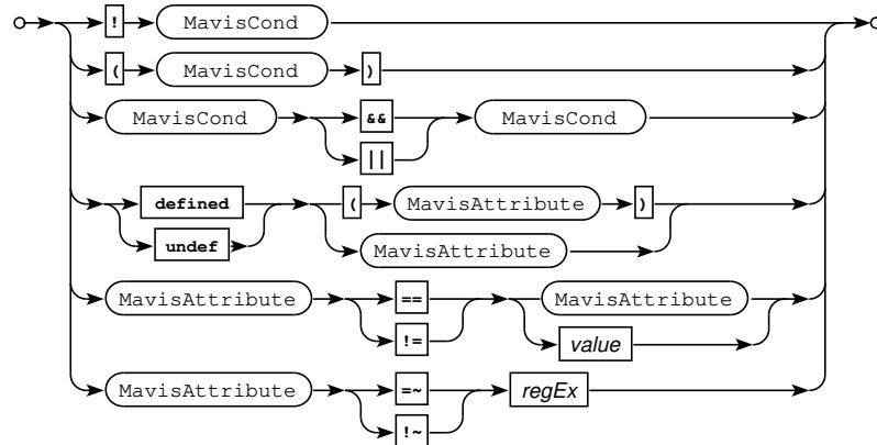
Railroad diagram: MavisCond
