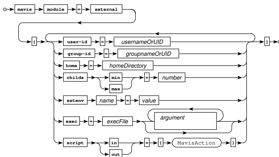
Railroad diagram: ExternalConf
