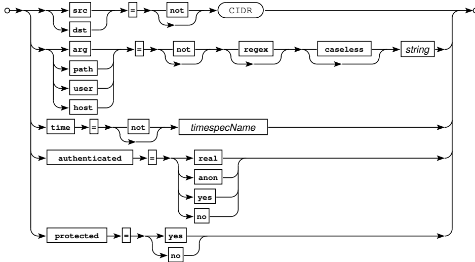
Railroad diagram: AclExpr
