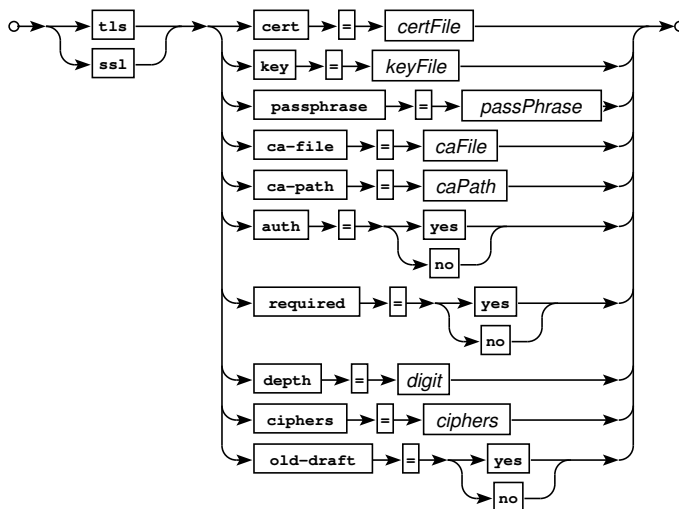
Railroad diagram: TLSExpr
