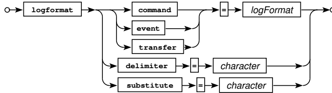
Railroad diagram: LogFormatExpr
