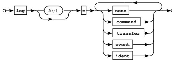
Railroad diagram: LogExpr
