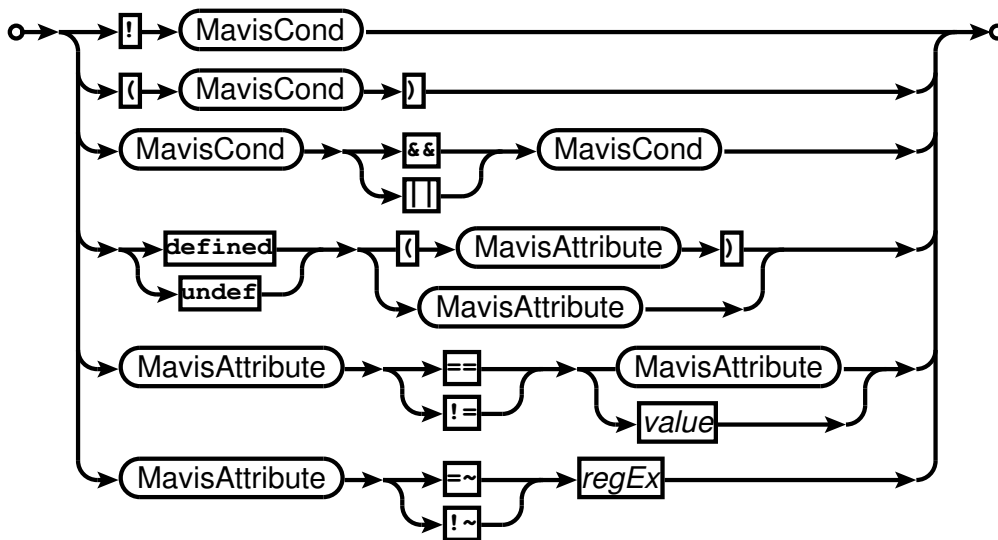
Railroad diagram: MavisCond
