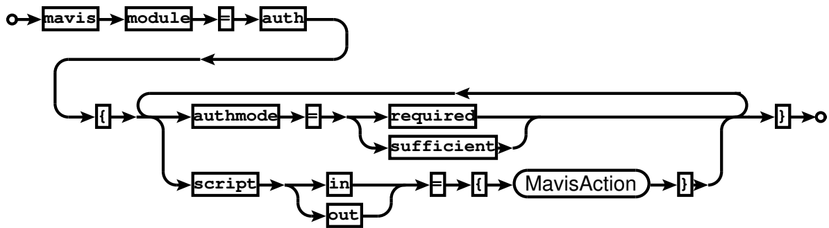
Railroad diagram: AuthConf
