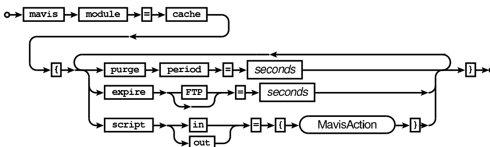
Railroad diagram: CacheConf
