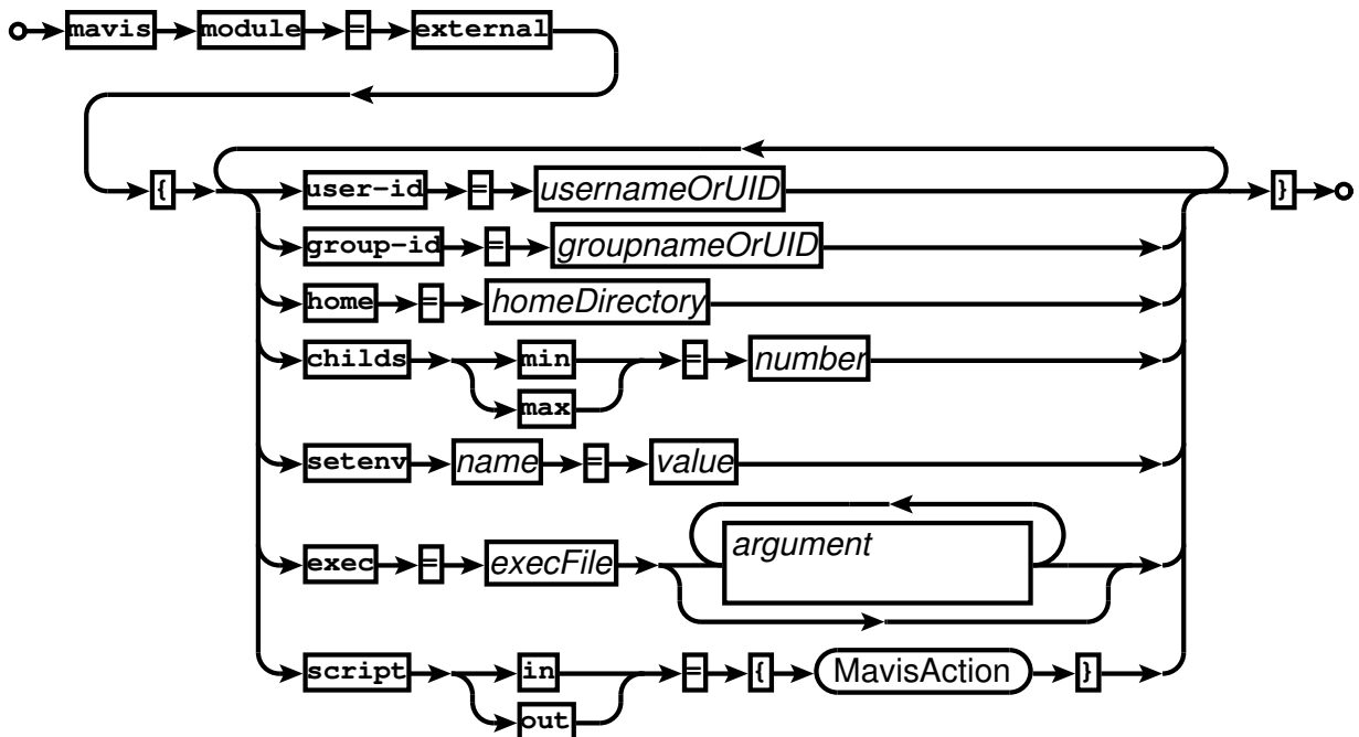
Railroad diagram: ExternalConf
