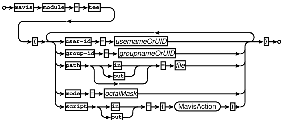
Railroad diagram: TeeConf
