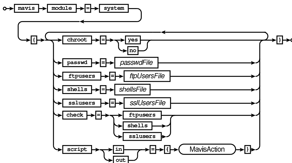
Railroad diagram: SystemConf
