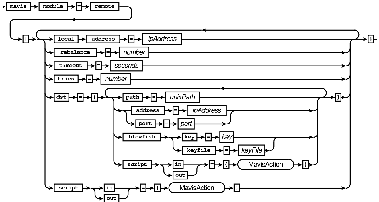
Railroad diagram: RemoteConf
