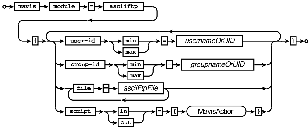
Railroad diagram: ASCIIftpConf
