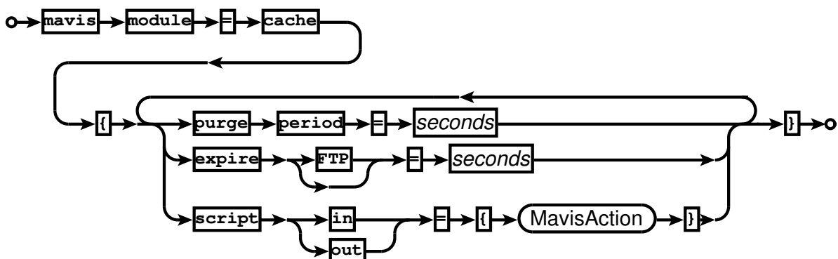
Railroad diagram: CacheConf
