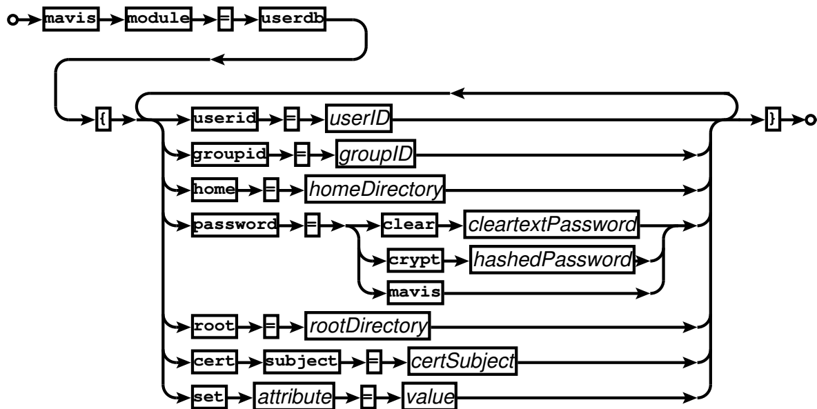
Railroad diagram: UserDBConf
