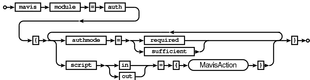
Railroad diagram: AuthConf
