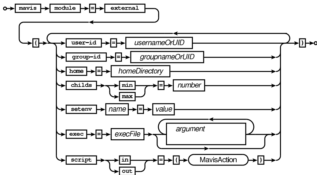
Railroad diagram: ExternalConf
