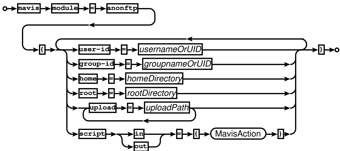
Railroad diagram: AnonftpConf
