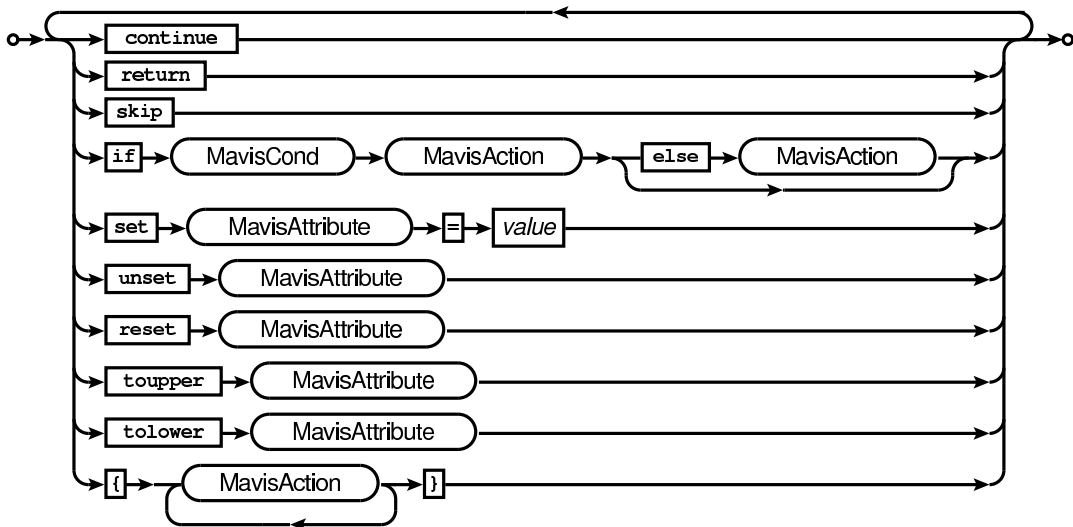
Railroad diagram: MavisAction
