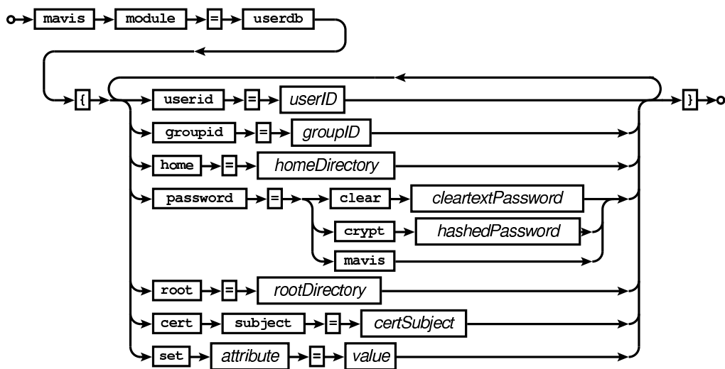
Railroad diagram: UserDBConf
