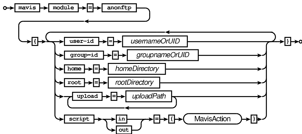
Railroad diagram: AnonftpConf
