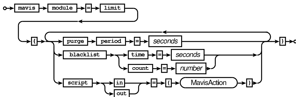
Railroad diagram: LimitConf
