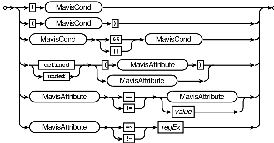
Railroad diagram: MavisCond
