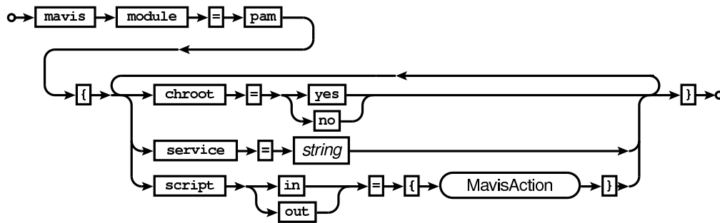
Railroad diagram: PAMConf
