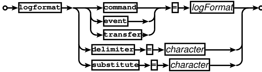
Railroad diagram: LogFormatExpr
