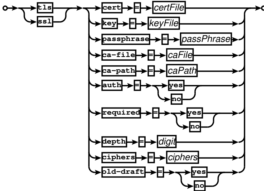
Railroad diagram: TLSExpr
