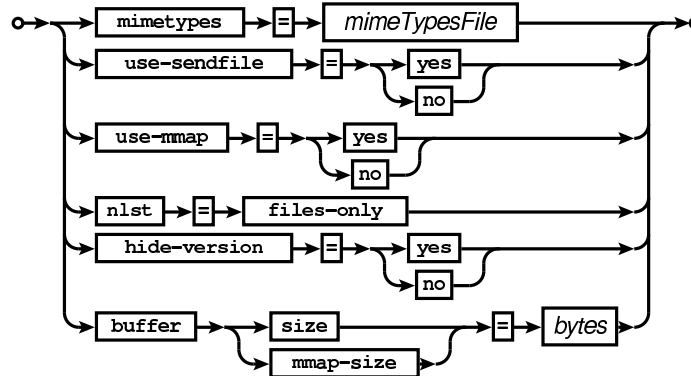
Railroad diagram: GlobalDecl
