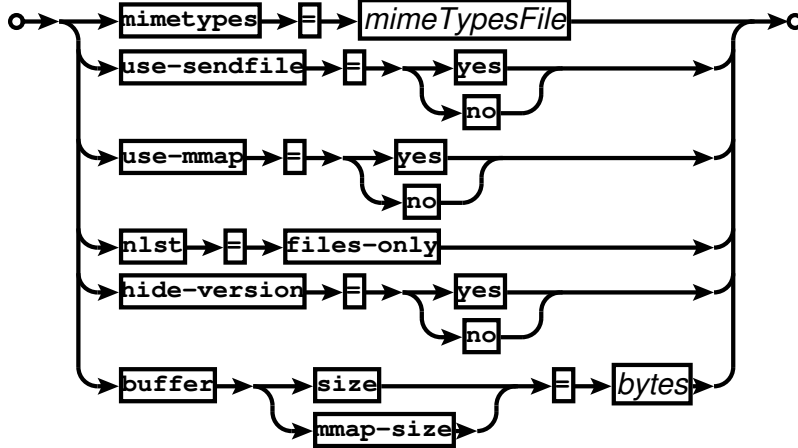
Railroad diagram: GlobalDecl
