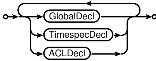
Railroad diagram: FtpdConfig
