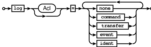
Railroad diagram: LogExpr
