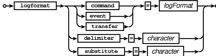
Railroad diagram: LogFormatExpr
