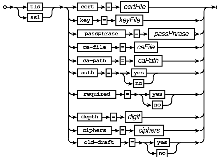
Railroad diagram: TLSExpr
