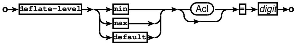
Railroad diagram: DeflateLevelExpr
