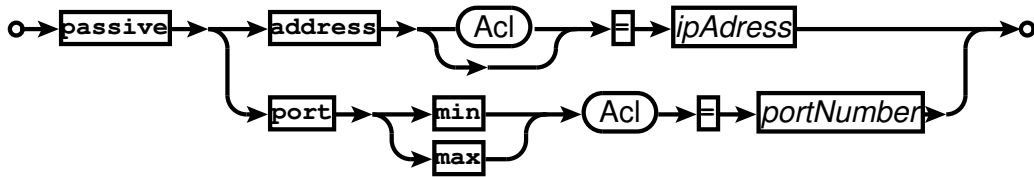
Railroad diagram: PassiveExpr
