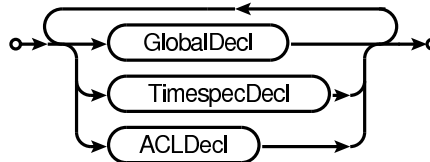
Railroad diagram: FtpdConfig
