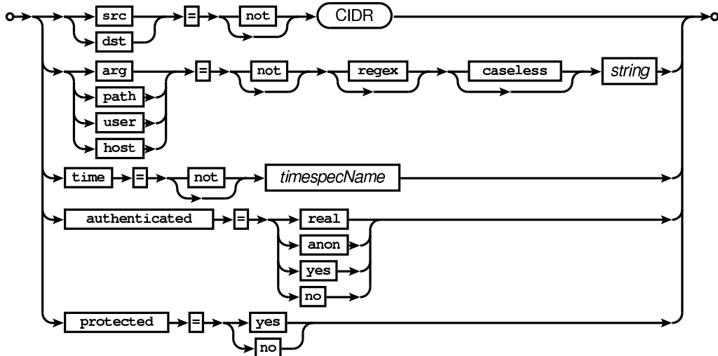
Railroad diagram: AclExpr
