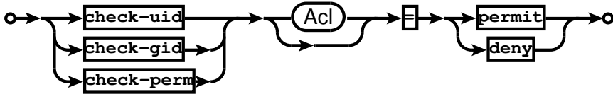
Railroad diagram: CheckExpr
