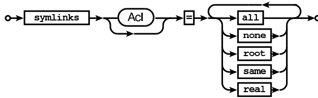
Railroad diagram: SymlinksExpr
