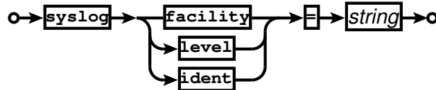
Railroad diagram: SyslogExpr
