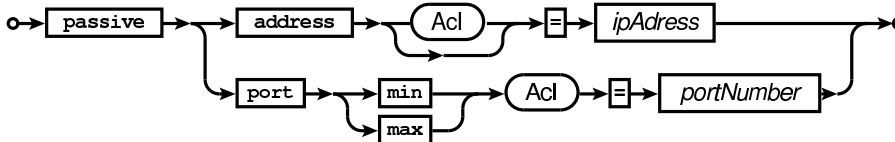
Railroad diagram: PassiveExpr
